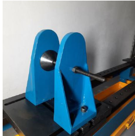
Clevis Support
